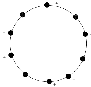
Figure 1.4: Ising Model
