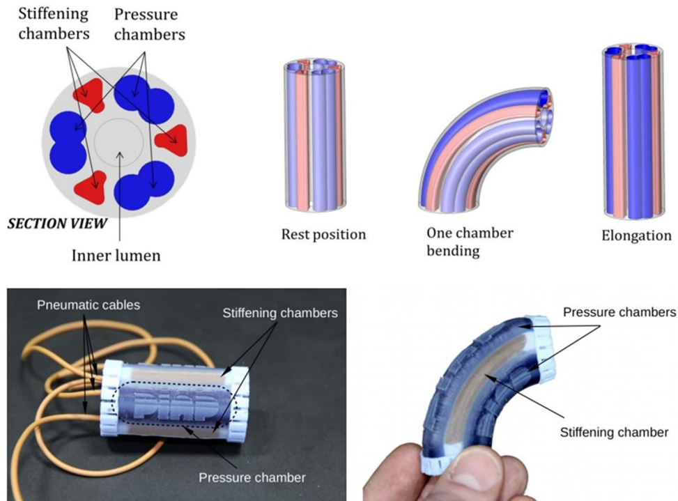
Fig. 1 Computer model design of one STIFF-FLOP arm segment. From the left Section view of the segment showing the arrangement of the chambers (pneumatic and stiffening); segment in the rest position (no pressure is supplied to the chambers); bending of the segment due to the pressurization of one pneumatic chamber (in dark blue); elongation of the segment due to the simultaneous pressurization of all the chambers. The stiffening mechanism can be activated by controlling the level of vacuum in all the stiffening chambers (in red), once the desired position of the segment is reached.
