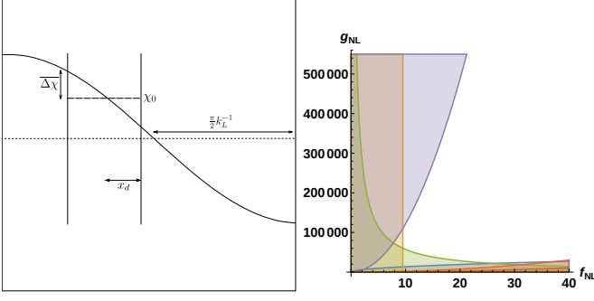
Figure 1. Left : The value of \chi varies by an amount \overline{\Delta\chi} from its average value, \chi_0 , within our observable universe (the interior of the two vertical lines), due to the long-wavelength fluctuation (solid wave). The average within our observable universe (long-dashed line) is not necessarily the same as the background value over the entire universe (dotted horizontal line). Right : Exclusion plot for (22)-dark-blue, (23)-orange, (24)-green, (25)-red, (26)-purple, (27)-brown, with x = 0.07 , a = 10 , b = 0.25 and c = 1 . The red and brown lines are hard to see on this scale at the bottom of the plot. The allowed region is left white.
