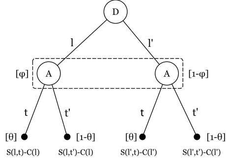
Figure 1: Game tree for the control game with 2 implementation levels and two targets.
