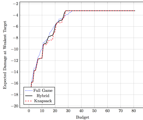
Figure 2: Comparison of Full Game, Hybrid and Pure Knapsack Methods of Decision Support.
