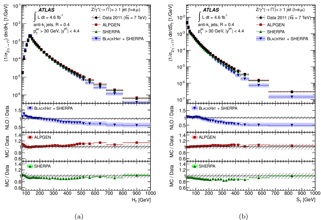
Figure 15. (a) Measured cross section for Z(\rightarrow \ell\ell)+\text{jets} as a function of the scalar p_T sum of the leptons and the jets, H_T , and (b) as a function of the scalar p_T sum of the jets, S_T , in events with at least one jet with p_T^{\text{jet}} > 30 GeV and |y^{\text{jet}}| < 4.4 in the final state. The cross sections are normalized to the inclusive Z(\rightarrow \ell\ell) cross section. The other details are as in figure 2.
