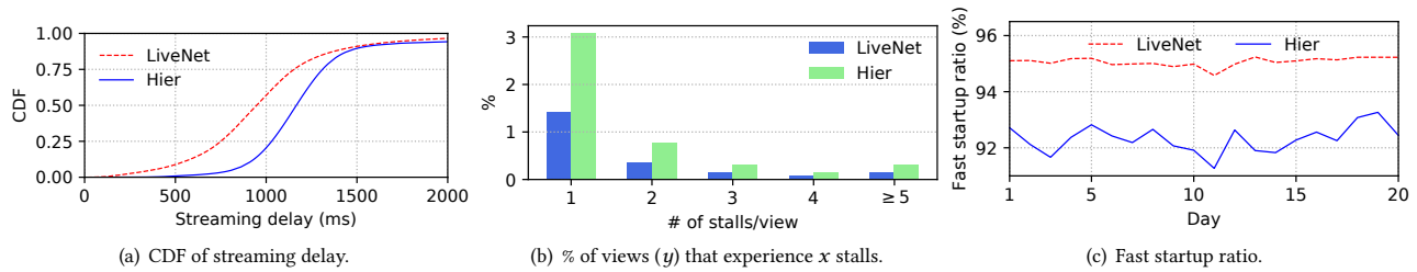
Figure 8: QoE metric comparison between LIVE NET and HIER.
