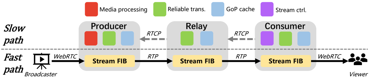
Figure 6: Transmission architecture overview.
