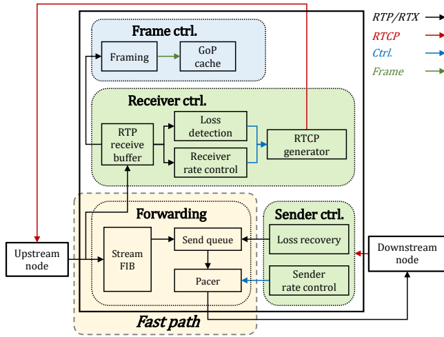
Figure 7: The software stack on overlay nodes for fast-slow path design.
