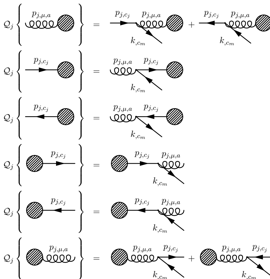
Figure 3. Action of the quark emission operator Q_j on an external parton line j , where all possible cases of incoming or outgoing line, and all parton species are considered. All momenta are defined to flow from left to right. The explicit contributions to the amplitude from each possibility are collected in appendix A.
