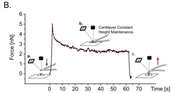
Fig. 1 Representation of an atomic force microscopy experiment. (A) Graphical explanation of an AFM experiment. The tip of the cantilever is positioned over the cell of interest (a.), moved along the Z-axis to indent the sample in the nuclear portion (b.) and then retracted (c.); the cantilever deflection is detected by a photodiode (PD). Plasticity index and work of adhesion were obtained by integrating the area between the approach and withdrawal curves, and are shown in the red and black dotted boxes, respectively. (B) Representative curve of a stress relaxation test performed on the nuclear region of cells. The tip of the cantilever approached the cell and indented it to 40% of its initial height (a.). The cantilever was maintained at the same height for a dwell period of 60 s (b.) and then retracted (c.). The dashed red line represents the bi-exponential fitting of the stress relaxation segment. (For interpretation of the references to color in this figure legend, the reader is referred to the web version of this article.)
