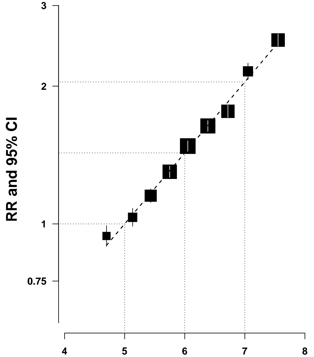
Logarithmic scale: linear association
