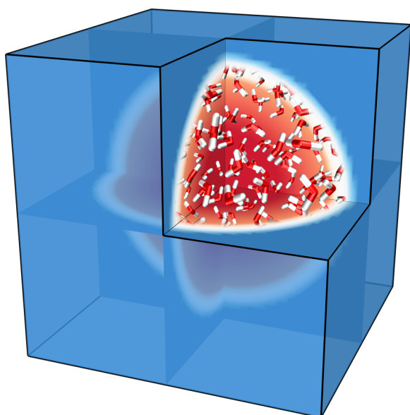
FIG. 1. Variable s parameter and MD sphere inside the computation box. The red zone is the pure MD region ( s = 0 ), while the blue is the fluctuating hydrodynamics region ( s = 1 ) for the spherically symmetrical s -function case.
