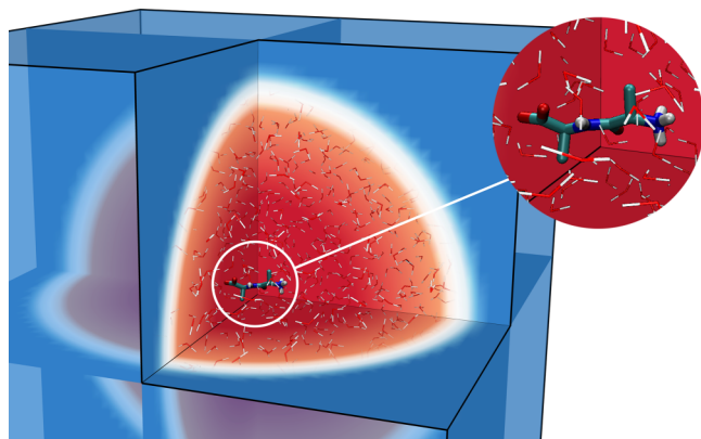
FIG. 18. Variable s parameter and MD sphere inside the computation box with a small peptide molecule, the zwitterionic form of dialanine, at the centre of the sphere. The red sphere is the pure MD region ( s = 0 ) and blue is the fluctuating hydrodynamics region ( s = 1 ).
