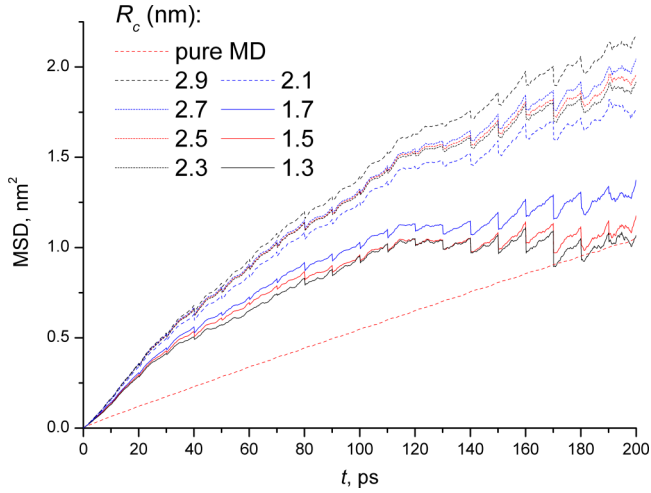
FIG. 21. The \text{MSD}(t) plots for protein (hybrid MD) calculated with different cutoff radii. The pure MD plot is given for comparison.
