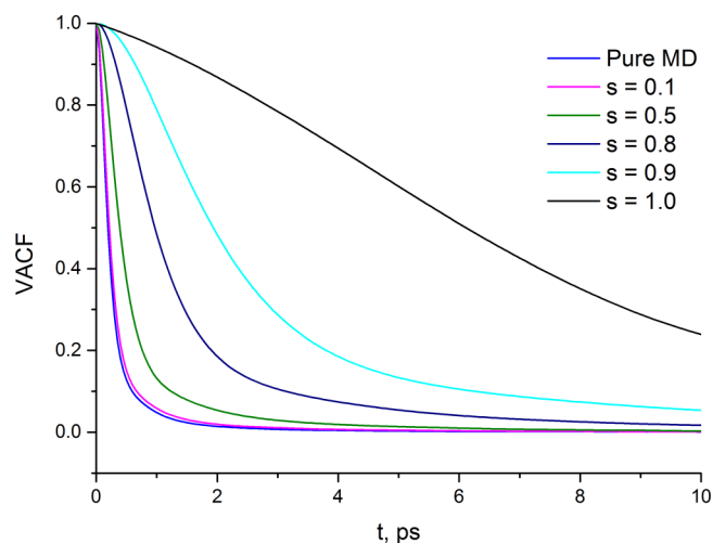
FIG. 5. Velocity autocorrelation functions for different constant s values for argon.
