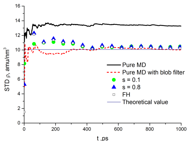
FIG. 7. Standard deviations of the density fluctuations for SPC/E water for five different cases: pure MD solution ( s = 0 ) without and with a blob filter, MD part of the solution for s = 0.1 and s = 0.8 , and LL-FH solution.
