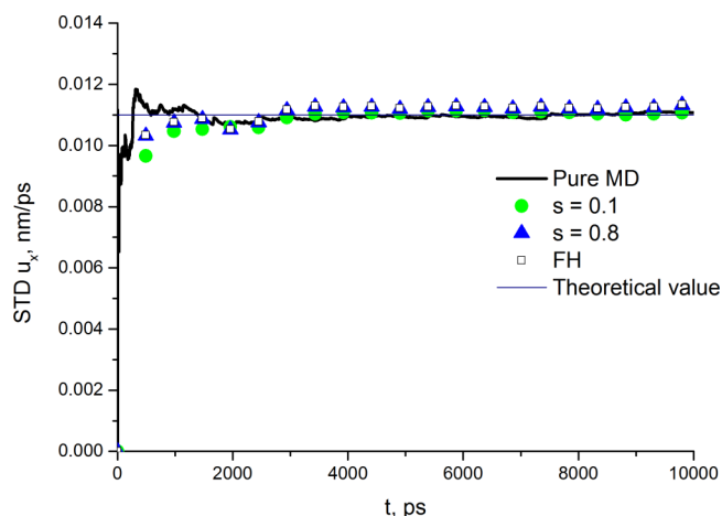
FIG. 2. Standard deviation of the velocity fluctuations for argon for four different cases: pure MD solution ( s=0 ) without a blob filter, MD part of the solution for s=0.1 and s=0.8 , and LL-FH solution.
