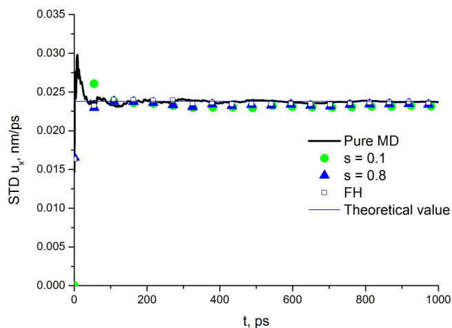
FIG. 6. Standard deviations of the velocity fluctuations for SPC/E water for four different cases: one pure MD case ( s = 0 ), two MD/LL-FH cases with s = 0.1 and s = 0.8 , and pure LL-FH case ( s = 1 ).
