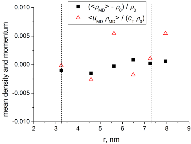
FIG. 14. Variation of time averaged density and momentum across the hybrid zone 0 < s < 1 shown by the vertical dotted lines (left, s = 0 and right, s = 1 ) for argon.
