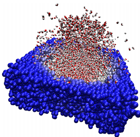
FIG. 9. A cross section of the simulation box with SPC/E water in the case of the variable s simulation; the white and red molecules are water molecules in the MD region and the blue spheres are the water blobs in the region dominated by hydrodynamics.
