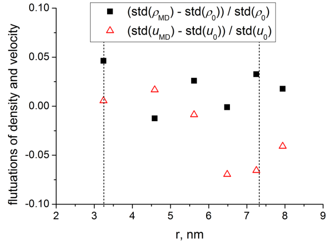
FIG. 15. Variation of standard deviation of density and momentum across the hybrid zone 0 < s < 1 shown by the vertical dotted lines (left, s = 0 and right, s = 1 ) for argon.
