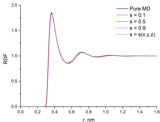
FIG. 4. Radial distribution functions for different s values for argon.
