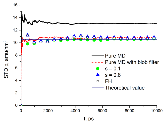
FIG. 3. Standard deviations of the density fluctuations for argon for five different cases: pure MD solution ( s=0 ) without and with a blob filter, MD part of the solution for s=0.1 and s=0.8 , and LL-FH solution.
