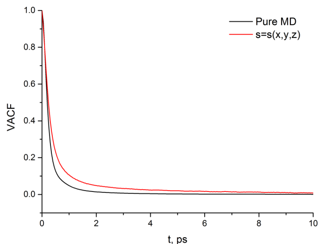
FIG. 8. Velocity autocorrelation functions in the case of variable s for argon.
