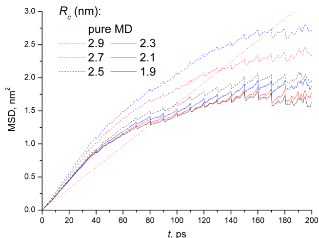
FIG. 20. The \text{MSD}(t) plots for water (hybrid MD) calculated with different cutoff radii. The pure MD plot is given for comparison.
