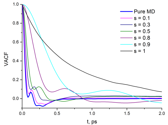
FIG. 12. Velocity autocorrelation functions for different constant s values for SPC/E water.
