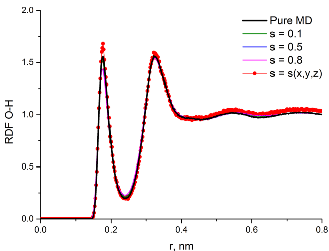
FIG. 11. Radial distribution functions oxygen-hydrogen for different s values for SPC/E water.
