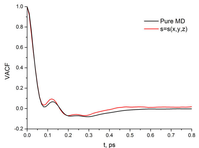
FIG. 13. Velocity autocorrelation functions in the case of variable s for SPC/E water.
