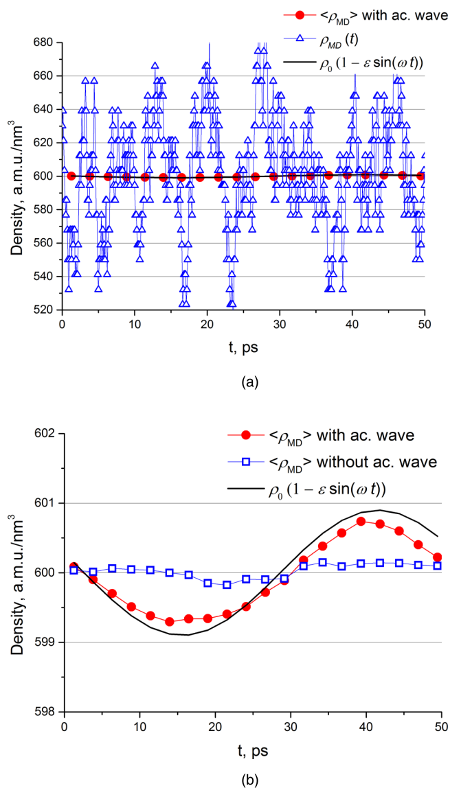
FIG. 17. Fluctuating density signal obtained in the MD part of the solution domain vs the analytical solution (a) including the original MD signal without phase and space averaging and (b) zoomed-in view with including the reference phase and space averaged solution without the acoustic wave.
