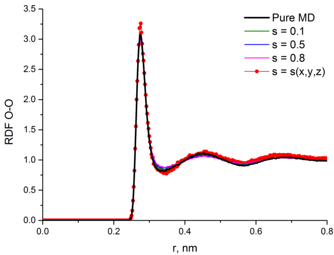
FIG. 10. Radial distribution functions oxygen-oxygen for different s values for SPC/E water.
