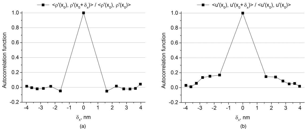
FIG. 16. Autocorrelations of (a) density and (b) x -velocity component for argon for the location x_0 at the centre of the hybrid MD/LL-FH zone.
