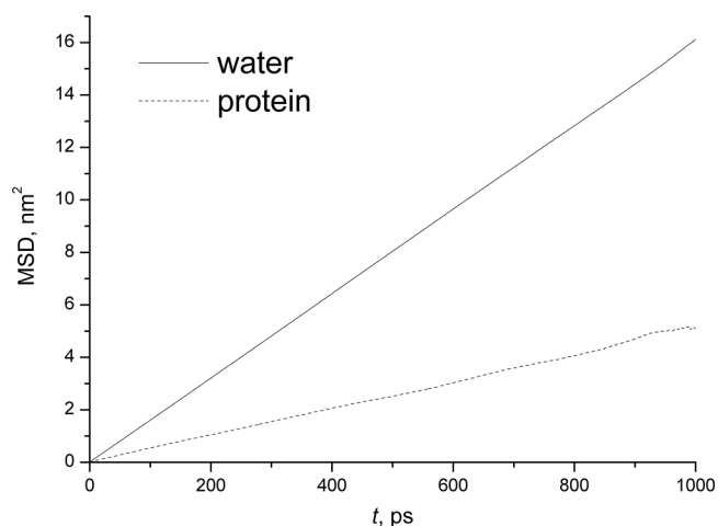
FIG. 19. The \text{MSD}(t) plot for the SPC/E water and the protein from a pure MD simulation.
