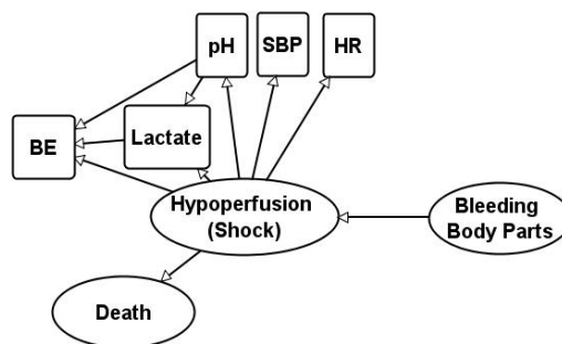
Figure 7.15 BN Structure after Node Merging
