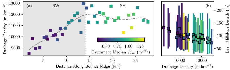
Figure 4: (a) Variation in catchment drainage density along the length of the Bolinas Ridge from NW to SE (distance from Point Reyes Station), color-coded by catchment-median channel steepness index ( \theta_{ref}=0.31 ). D_D increases with distance until \sim 15 km along the landform. (b) Variation in hillslope length (median and 16th–84th percentile range L_H ) with D_D showing an inverse relationship.
