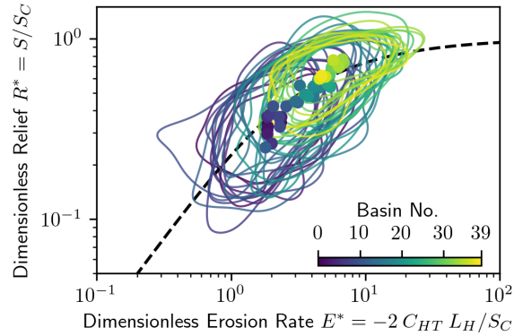
Figure 9: Plot showing the progression of hillslope morphology along the length of the Bolinas Ridge. Colored lines are the 90th percentile contour of E^* vs R^* point density for traces within each catchment, where catchment numbers increase from NW to SE. Points are the median values in each catchment.
