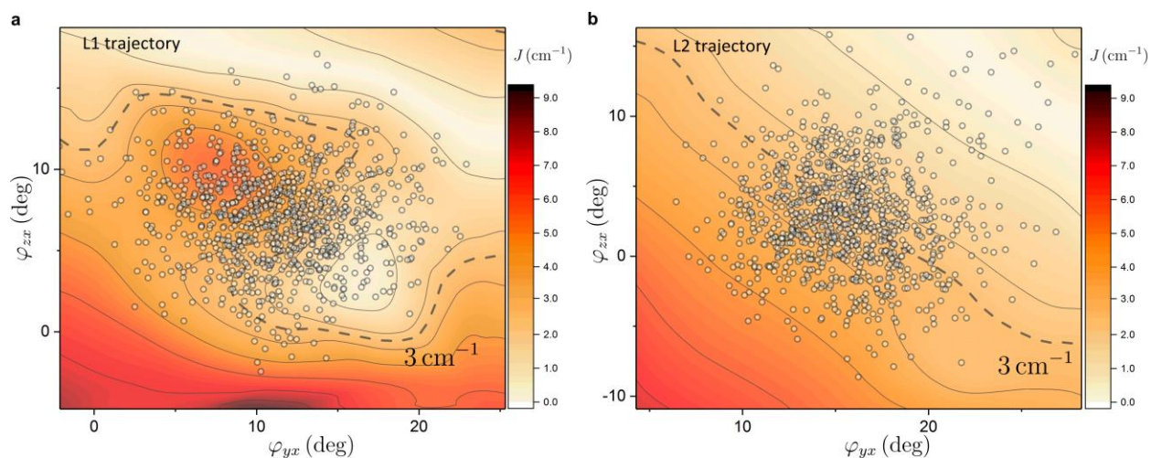
Figure 4 | The Chl Q_y and Car S_1 state interaction energy surfaces. (a,b) The IES (absolute values) are shown for the L1 and L2 sites, respectively. The white circles represent the actual values of the two angles from the MD trajectory. The dashed lines show the J = 3 \text{ cm}^{-1} values for guidance. For the interpolation of the 41 TDC coupling values a 100 \times 100 point grid was used.
