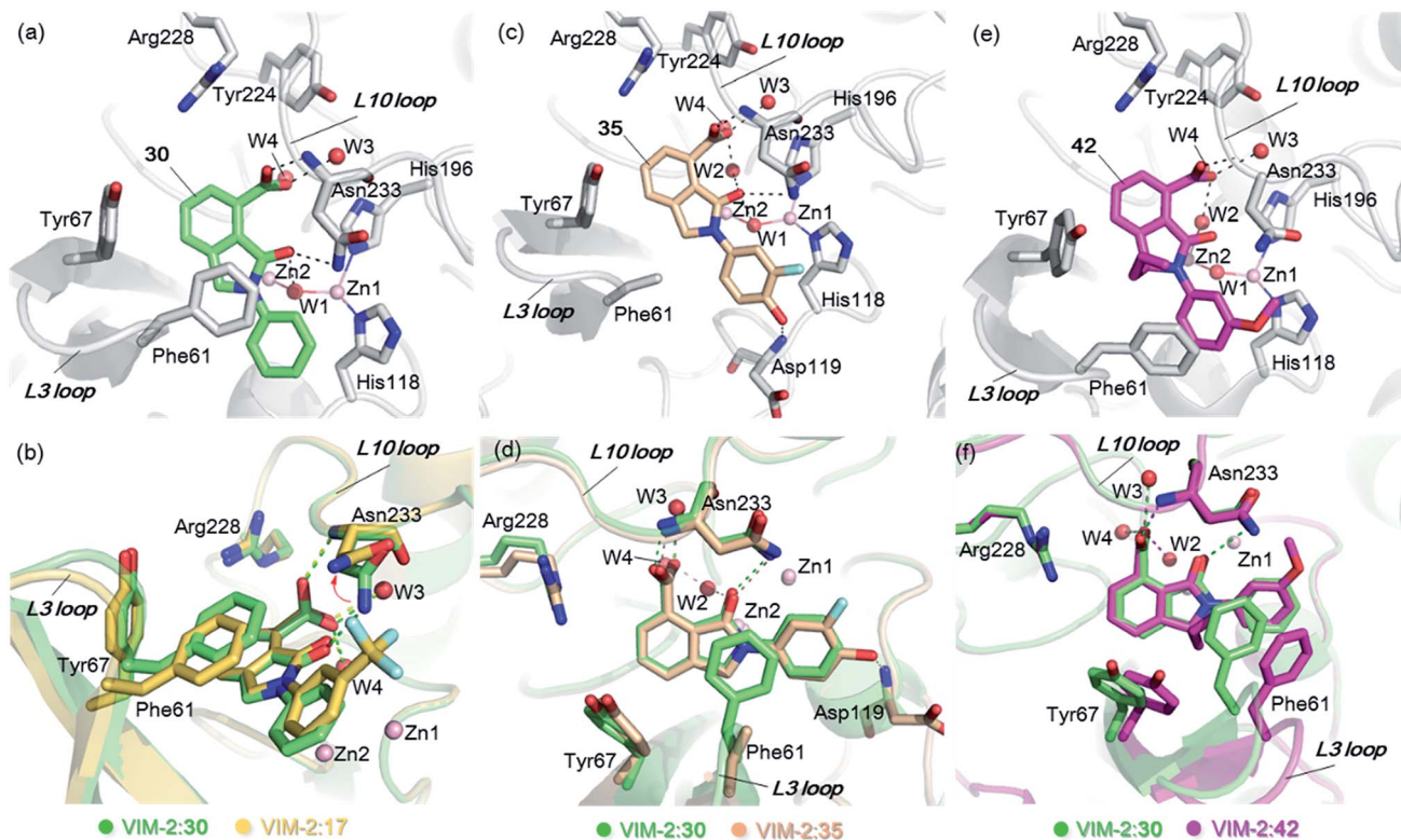
Fig. 5 Crystallographic analyses reveals how the 3-oxoisindoline-4-carboxylate derivatives bind to the VIM-2 MBL. (a) View from a crystal structure of VIM-2 in complex with 30 (PDB ID 5LFCF). (b) Comparison of structures of VIM-2:17 and VIM-2:30 reveals the Asn233 side chain is unable to form hydrogen-bonds with the 3-oxoisindoline-4-carboxylate of 17 due to its trifluoromethyl group, which may explain why 17 is less potent than 30 (Table 2). (c) View from a crystal structure of VIM-2 in complex with 35 (PDB ID 5LM6). (d) Comparison of VIM-2:30 and VIM-2:35 complex structures reveals 30 and 35 have the same binding mode. (e) View from a crystal structure of VIM-2 in complex with 42 (PDB ID 5LCH). (f) Comparison of structures of VIM-2:30 and VIM-2:42 reveals evidence for flexibility in the conformation of Tyr67 and Phe61 on the L3 loop, suggesting Tyr67 and Phe61 may play important roles in capturing substrates and delivering them to the zinc ions for hydrolysis.
