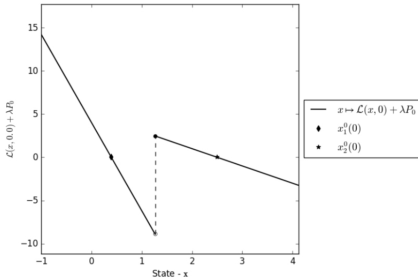
(a) Illustration when c = 0
