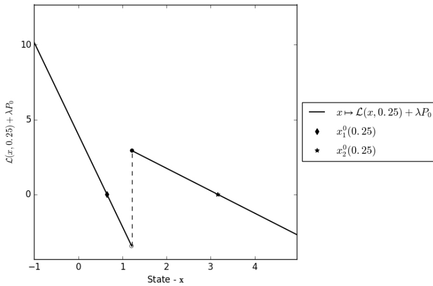
(b) Illustration when c = 0.25
