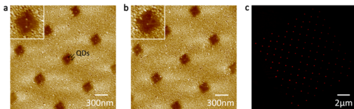
Figure 3. Images of the assembly of QDs in nanoarrays via the covalent immobilisation of QD-labelled triangular DNA origami in pre-patterned nanoapertures. (a) AFM image for the case of 3 QDs per origami, and hence per aperture; (b) AFM image for the case of 2 QDs; (c) Epifluorescence microscopy image of a glass substrate patterned with 3 QDs per 1\mu\text{m} spaced nanoaperture: each nanoaperture is optically resolvable.
