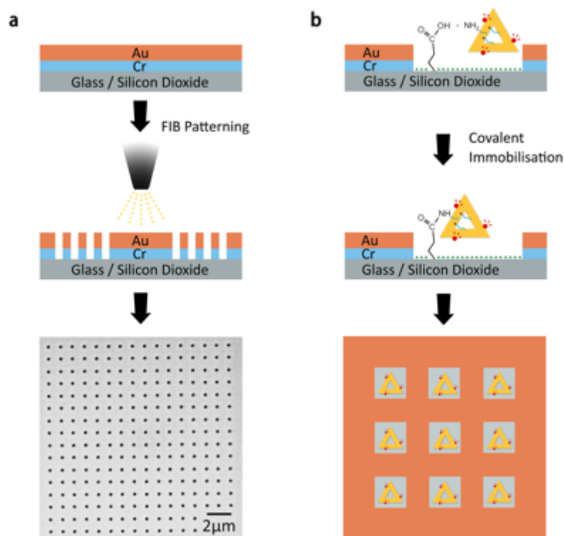
Figure 2. Schematic and images of the patterning and assembly process. (a) Schematic of the patterning to fabricate nanoaperture arrays and SEM image of the final substrate; (b) Schematic of the covalent immobilisation of amino-terminated and QD-labelled triangular DNA origami on patterned surfaces via amidation reactions.
