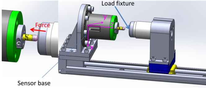
Fig. 10. Overview of calibration device designed by Solidworks to obtain the characteristic curve between the physical force F_z and the three light intensity values for the three optical fibers.
