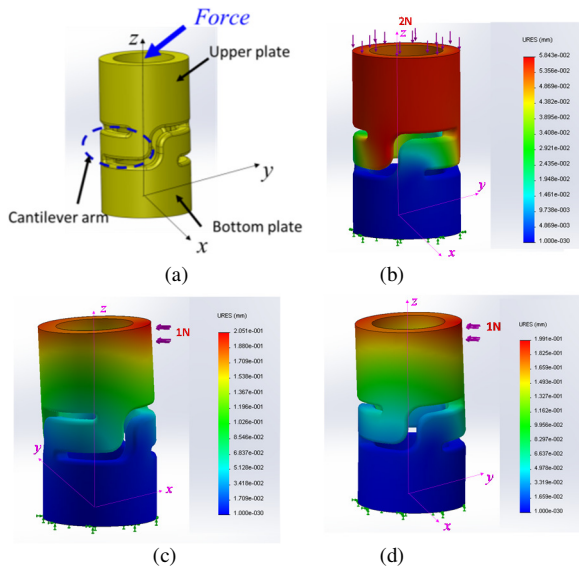
Fig. 7. FEA simulation of sensor mechanical structure using SolidWorks a) Sensor mechanical structure b) Maximum deflection when F_z is applied along z-axis c) Maximum deflection when F_x is applied along x-axis d) Maximum deflection when F_y is applied along y-axis
