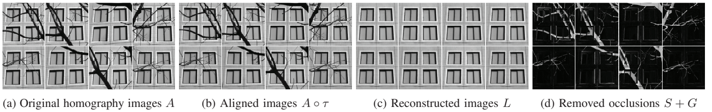
Figure 4: Alignment and recovery of planar homographies.
