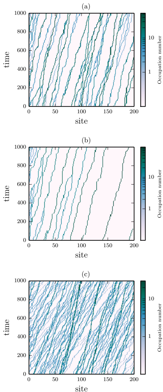
FIG. 2. (Color online) Monte Carlo time evolution of the occupation profile of the on-off ZRP on a one-dimensional lattice. (a) Rates \mu_{n,\tau} = n if \tau > 0 , \mu_{n,\tau} = 0 otherwise, and (\alpha, \beta, \gamma, \delta, p, q, c) = (0.1, 0.2, 0, 0, 1, 0, 0.05) . Only correlations due to the blockade mechanism are present. The particles organise in travelling clusters. Their speed is mainly governed by c . (b) Same parameters as the former case, except (\beta, p) = (10^4, 10^4) . The particles jump almost simultaneously to the next site as soon as the blockade is removed. Each particle cluster tends to occupy a single site. The drift proceeds with a rate \simeq c . (c) Same parameters as (a), except \mu_{n,\tau} = 1 if \tau > 0 and n > 0 , \mu_{n,\tau} = 0 otherwise, and c = 0.15 . As a result of the attractive inter-particle interaction, the clusters with more particles travel slower than the less populated ones. This mechanism enhances congestion.
